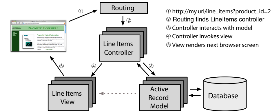
Figure 5—Rails and MVC
