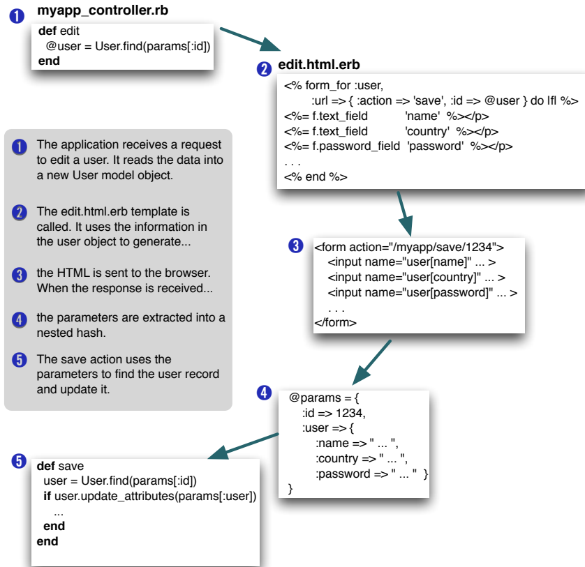
Figure 50—Models, controllers, and views work together.
