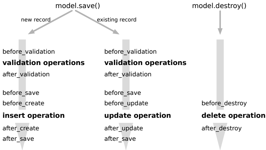
Figure 48—Sequencing of Active Record callbacks
