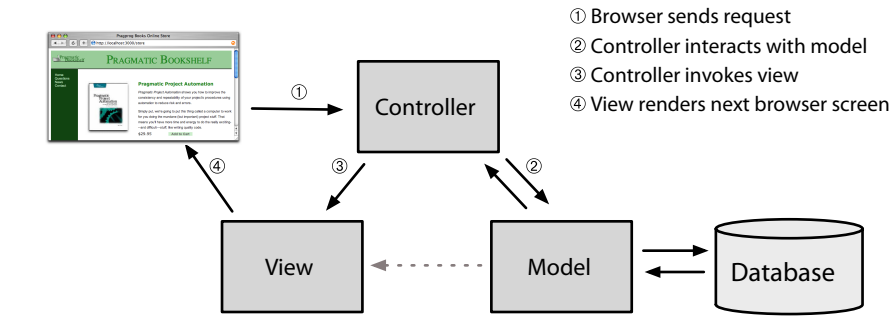
Figure 4—The Model-View-Controller architecture
